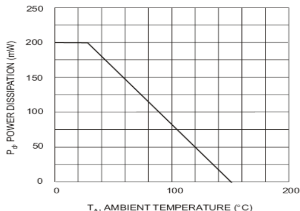
Fig. 4 Power Derating Curve, Total Package
